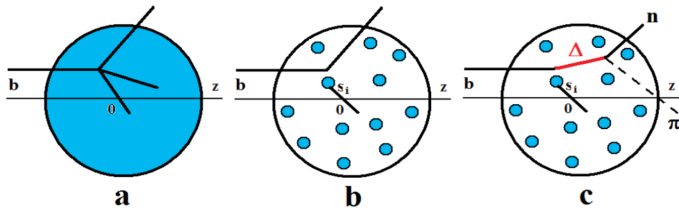
Fig. 25.15: Cascade-type sampling.
