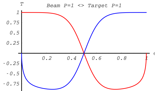
Fig. 13.8: Polarization transfer functions in Møller scattering. Longitudinal polarization \xi_3^{(2)} of electron with energy E_{p_2} in blue; longitudinal polarization \xi_3^{(1)} of second electron in red. Kinetic energy of incoming electron T_{k_1} = 10\text{MeV}
