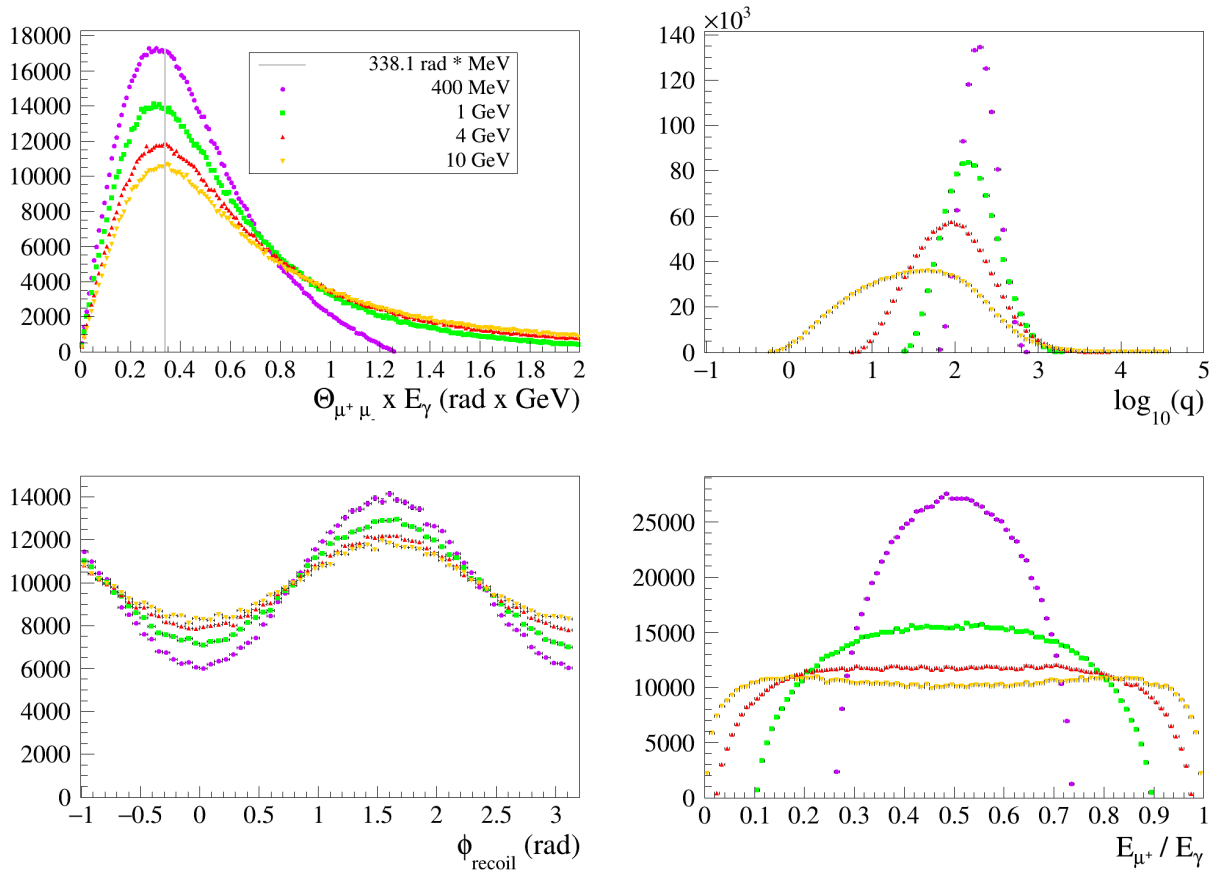
Fig. 6.16: G4BetheHeitler5DModel : \gamma -ray conversions to \mu^+\mu^- pairs on Argon atoms (see text), for various incident-photon energies (bullets 400 MeV, squares 1 GeV, upper triangle 4 GeV, down triangle 10 GeV).
