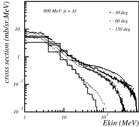
Fig. 27.4: Double differential cross-section for neutrons produced in proton scattering off Aluminum. Proton incident energy was 800 MeV. The points are data, the histogram is Binary Cascade prediction.
