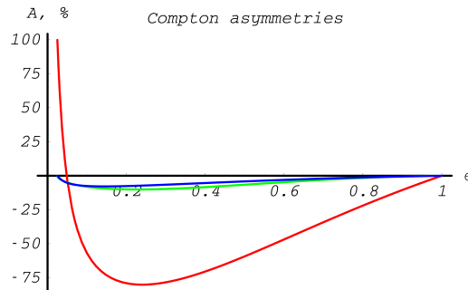
Fig. 13.20: Compton scattering differential cross section asymmetries in%. Red line corresponds to the asymmetry due to circular photon and longitudinal electron initial state polarization, green line – due to circular photon and transverse electron initial state polarization, blue line – due to linear photon and transverse electron initial state polarization.
