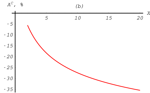
Fig. 13.18: Compton total cross section asymmetry depending on the energy of incoming photon. Up to 10MeV.
