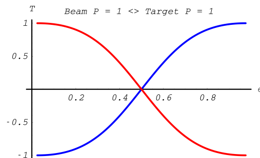
Fig. 13.15: Polarization Transfer in annihilation process. Blue line corresponds to the circular polarization \xi_3^{(1)} of the photon with energy m(\gamma + 1)\epsilon ; red line – circular polarization \xi_3^{(2)} of the photon photon with energy m(\gamma + 1)(1 - \epsilon) .
