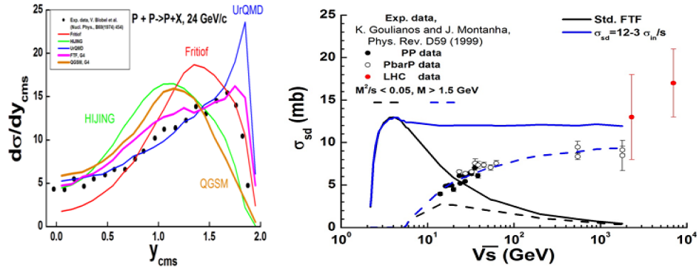
Fig. 25.11: Left: inclusive spectrum of proton in pp -interactions at P_{\text{lab}} = 24 \text{ GeV}/c . Points are experimental data [eal74], lines are model calculations. Right: single diffraction dissociation cross section in pp -interactions. Points are data gathered by K. Goulianos and J. Montanha [GM99]. Lines are FTF model calculations.
