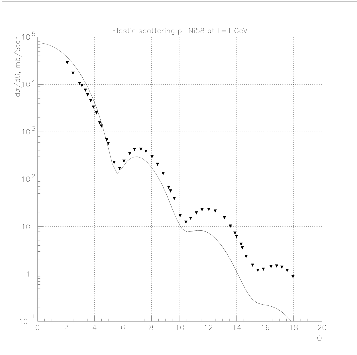
Fig. 23.7: Elastic proton scattering on 58 Ni at 1 GeV.
