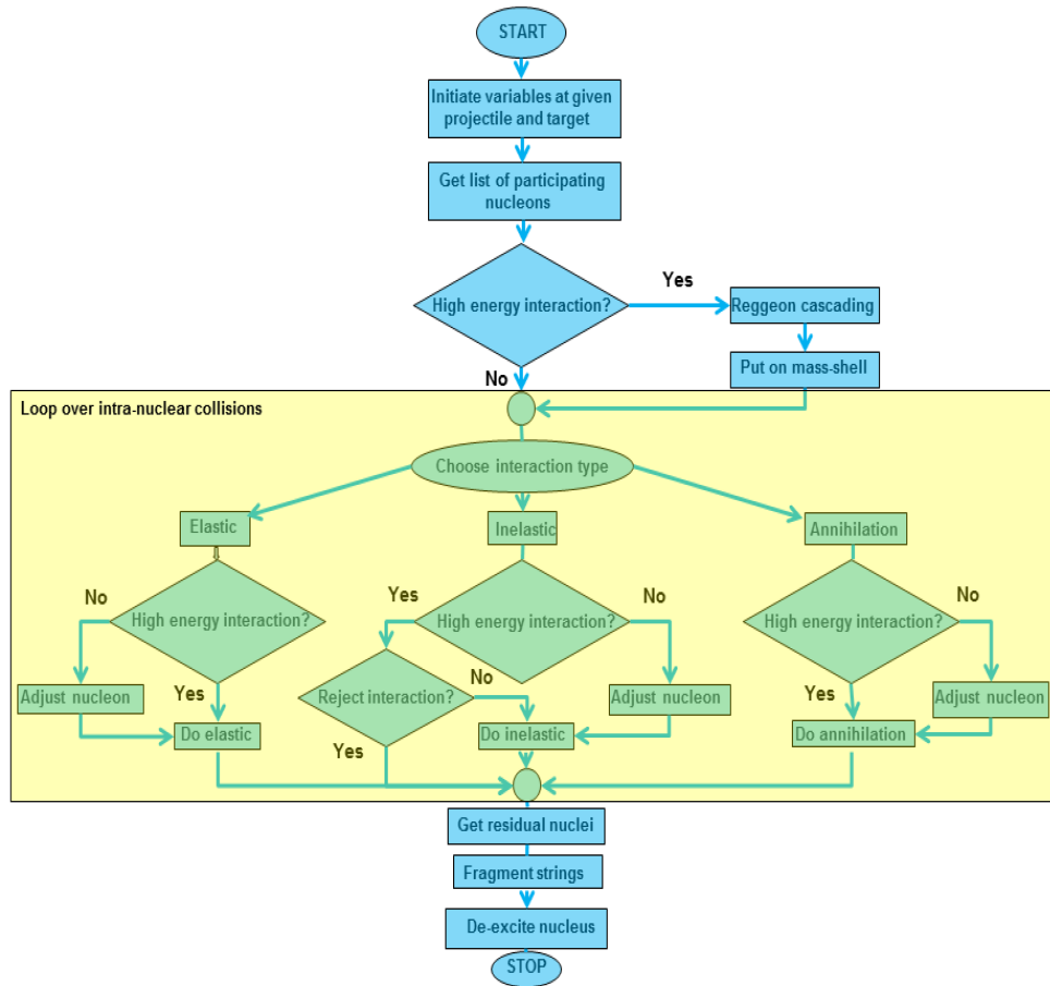
Fig. 25.14: Flowchart of the FTF model.
