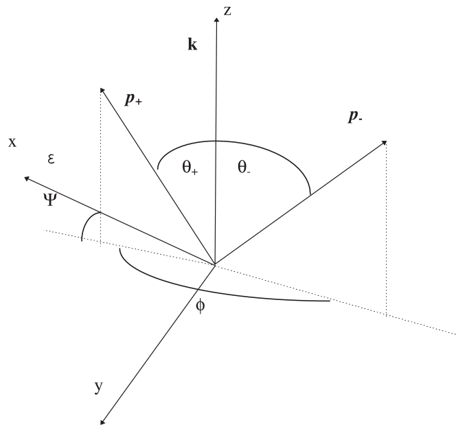
Fig. 13.24: Angles occurring in the pair creation
