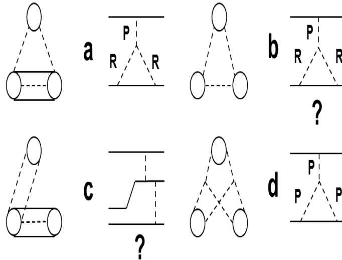
Fig. 25.21: Diagrams of quark-gluon exchanges and corresponding reggeon diagrams for hadron-nucleus interactions.
