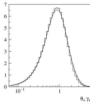
Fig. 6.14: Angular distribution in logarithmic scale. The curve corresponds to the exact calculations and the histogram is the simulated distribution.
