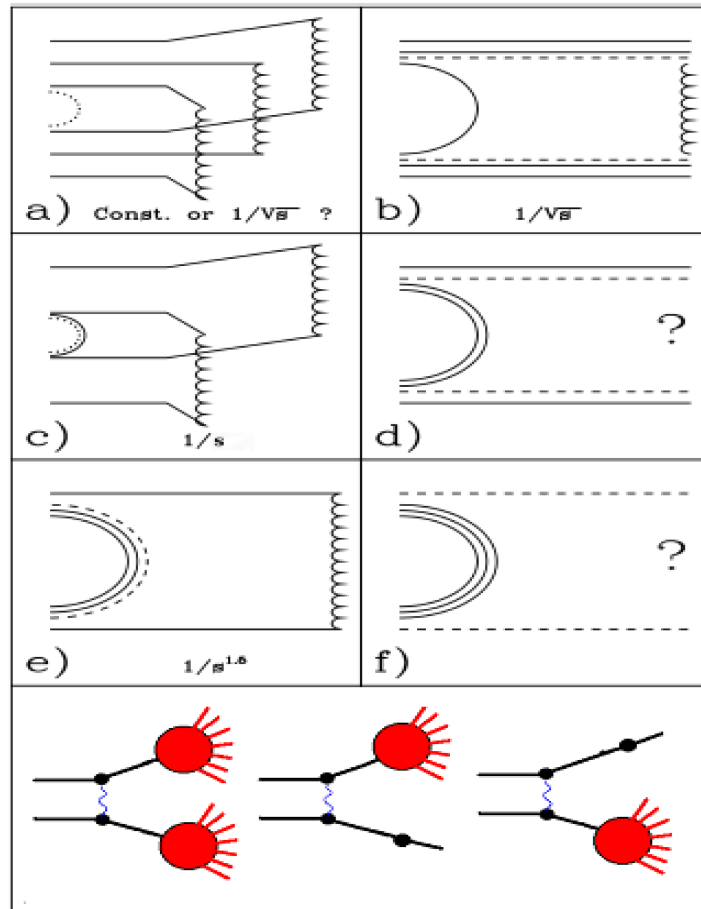
Fig. 25.10: Quark flow diagrams of \bar{p}p -interactions.
