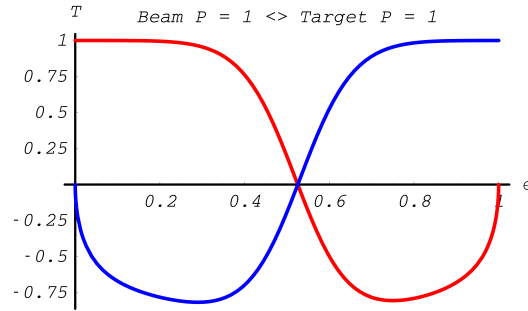
Fig. 13.10: Polarization Transfer in Bhabha scattering. Longitudinal polarization \xi_3^{(2)} of electron with energy E_{p_2} in blue; longitudinal polarization \xi_3^{(1)} of scattered positron. Kinetic energy of incoming positron T_{k_1} = 10\text{MeV}
