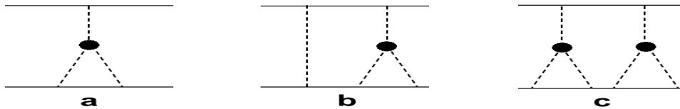
Fig. 25.17: Simplest enhanced diagrams of NN -scattering.
