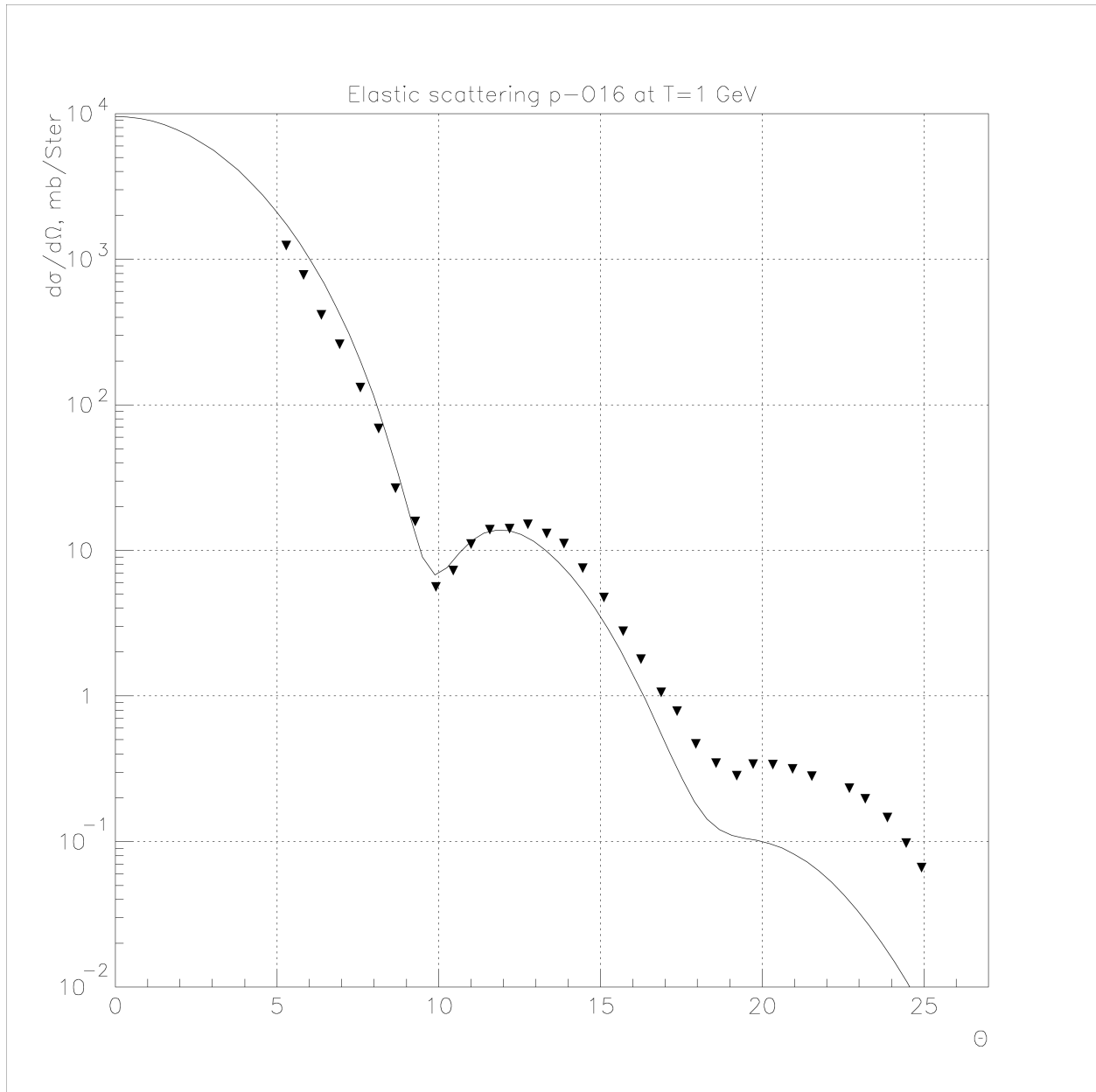
Fig. 23.4: Elastic proton scattering on ^{16}\text{O} at 1 GeV.
