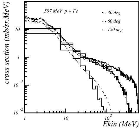
Fig. 27.7: Double differential cross-section for neutrons produced in proton scattering off Iron. Proton incident energy was 597 MeV. The points are data, the histogram is Binary Cascade prediction.
