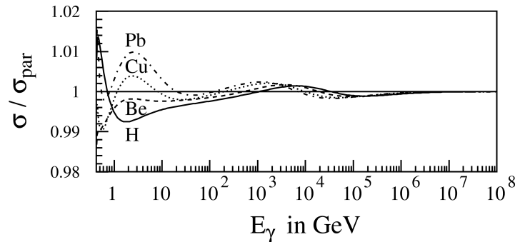
Fig. 6.5: Ratio of numerically integrated and parameterized total cross sections as a function of E_\gamma for hydrogen, beryllium, copper and lead.
