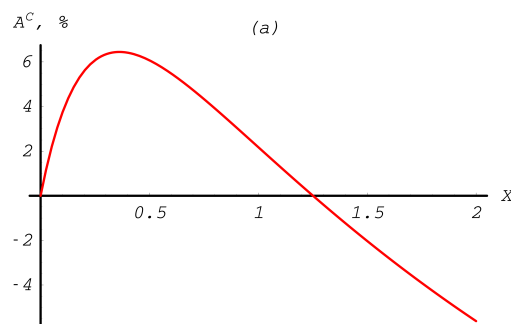
Fig. 13.17: Compton total cross section asymmetry depending on the energy of incoming photon. Between 0 and \sim 1 MeV.
