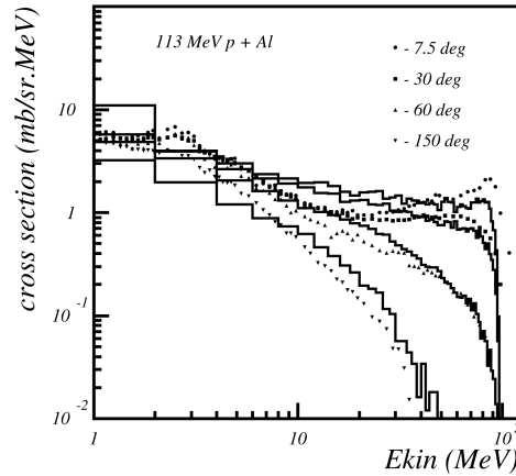
Fig. 27.1: Double differential cross-section for neutrons produced in proton scattering off Aluminum. Proton incident energy was 113 MeV.
