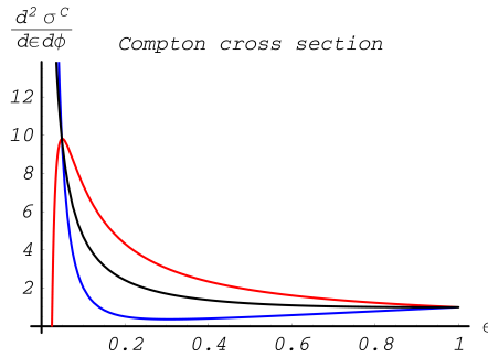
Fig. 13.19: Compton scattering differential cross section in arbitrary units. Black line corresponds to the unpolarized cross section; red line – to the antiparallel spins of initial particles, and blue line – to the parallel spins. Energy of the incoming photon E_{k_1} = 10\text{MeV} .
