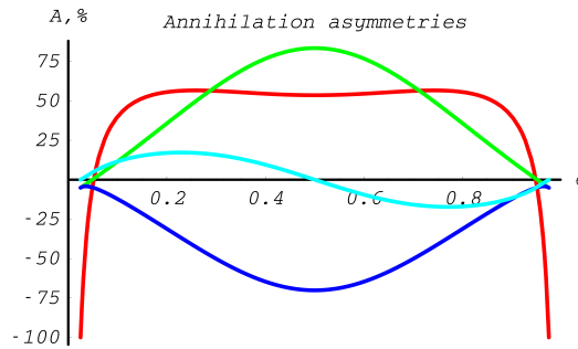
Fig. 13.14: Annihilation differential cross section asymmetries in %. Red line corresponds to A_{ZZ}(\epsilon) , green line – A_{XX}(\epsilon) , blue line – A_{YY}(\epsilon) , lightblue line – A_{ZX}(\epsilon) . Kinetic energy of the incoming positron T_{k_1} = 10\text{MeV} .
