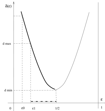
Fig. 6.2: Calculation of \epsilon for gamma conversion.
