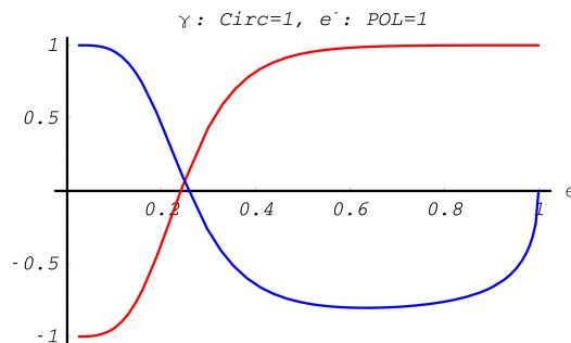
Fig. 13.21: Polarization Transfer in Compton scattering. Blue line corresponds to the longitudinal polarization \xi_3^{(2)} of the electron, red line – circular polarization \xi_3^{(1)} of the photon.
