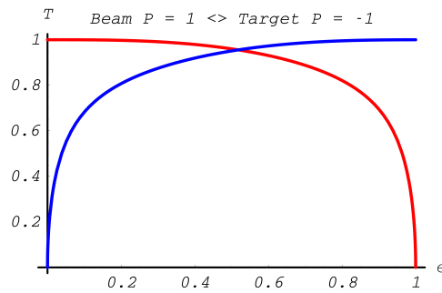
Fig. 13.11: Polarization Transfer in Bhabha scattering. Longitudinal polarization \xi_3^{(2)} of electron with energy E_{p_2} in blue; longitudinal polarization \xi_3^{(1)} of scattered positron. Kinetic energy of incoming positron T_{k_1} = 10\text{MeV}
