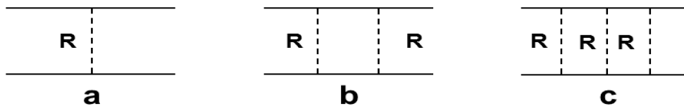
Fig. 25.16: Nonenhanced diagrams of NN -scattering.
