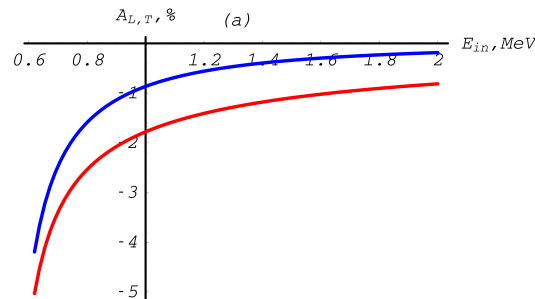
Fig. 13.2: Møller total cross section asymmetries depending on the total energy of the incoming electron, with a cut-off T_{\text{cut}} = 1 \text{ keV} . Transverse asymmetry is plotted in blue, longitudinal asymmetry in red. Between 0.5 MeV and 2 MeV.
