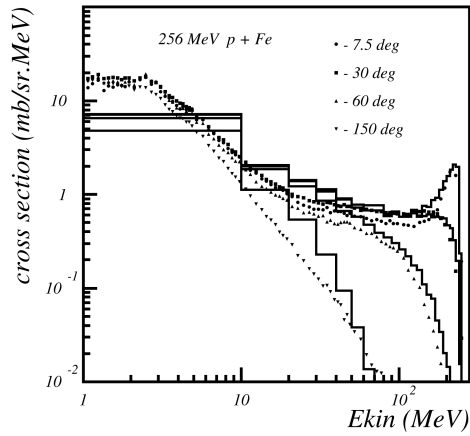
Fig. 27.6: Double differential cross-section for neutrons produced in proton scattering off Iron. Proton incident energy was 256 MeV. The points are data, the histogram is Binary Cascade prediction.
